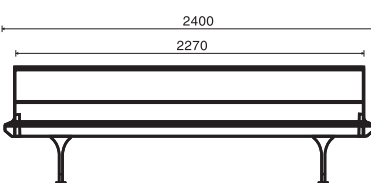
Model. SIVER SURF-03
